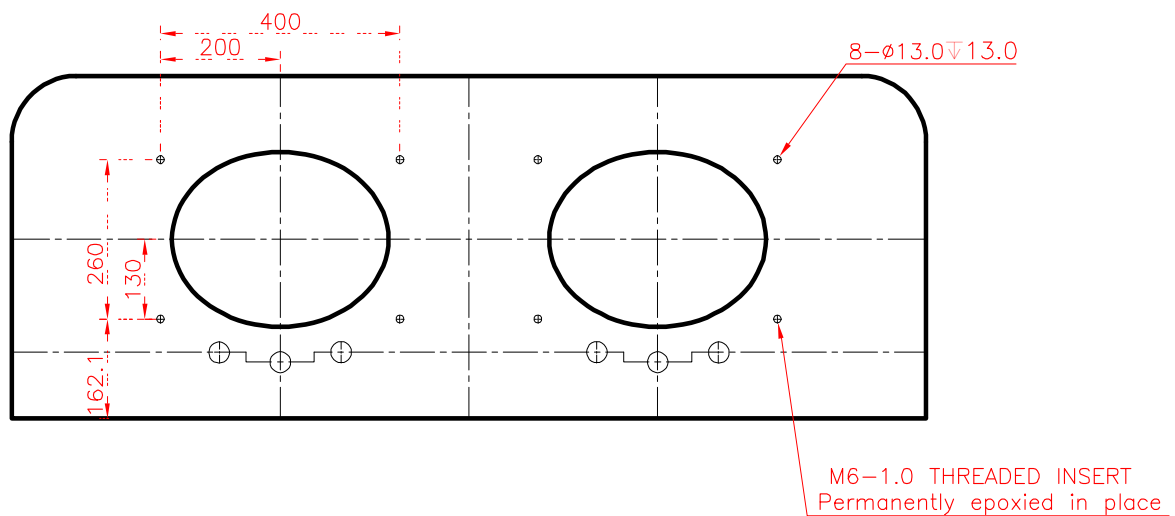
BOTTOM VIEW
