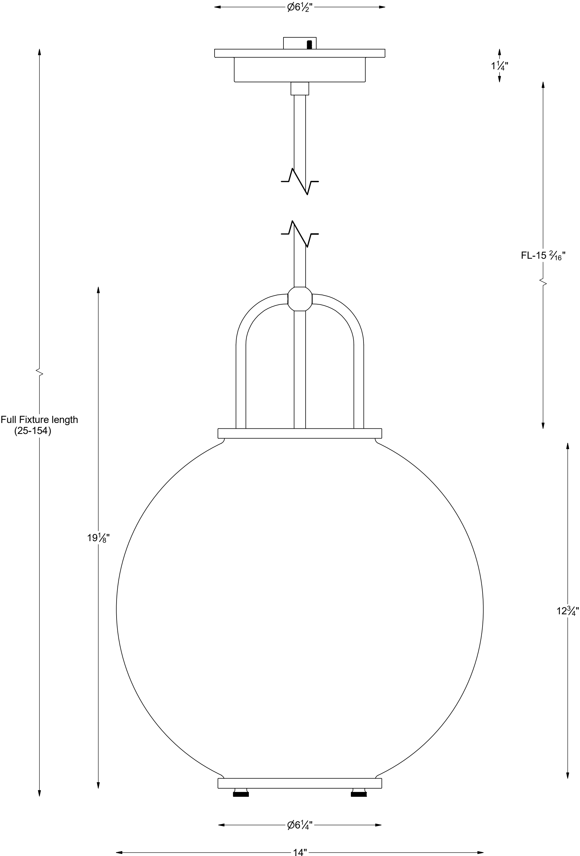
A1658 Yeon pendant globe 14in brass
