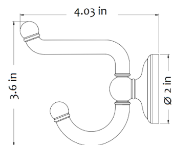
Double hook
