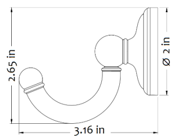
Single hook
