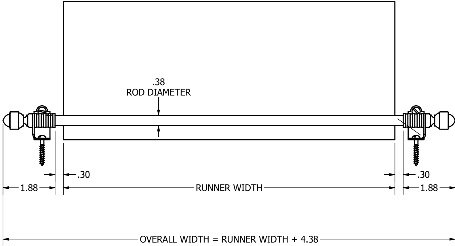
FRONT VIEW
