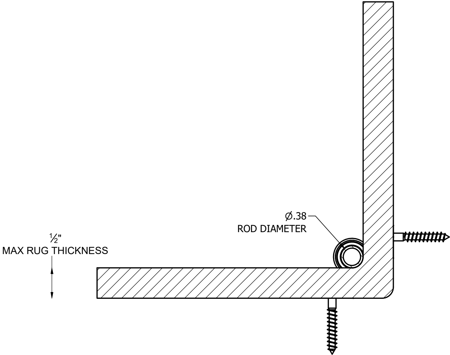
SIDE SECTION VIEW
