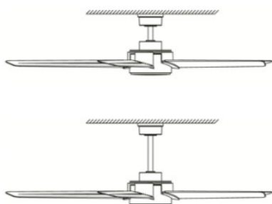
Downrod installation
