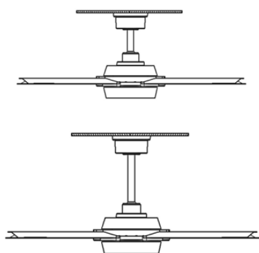
Downrod installation
