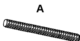
A Ø5/16" x 3" 8x
