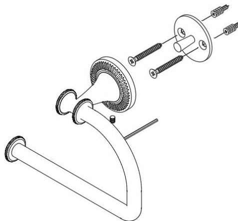
Installation de vis (sans ancrage)
