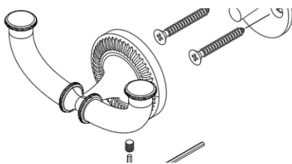
For stud mounting (no anchor)
