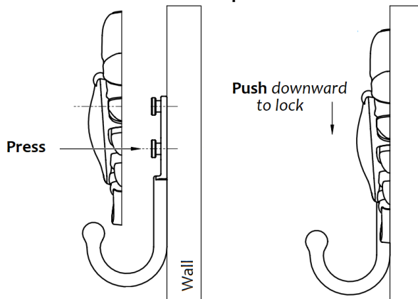
Fig. 3 Press decorative cover onto mounting bracket while pushing downward to lock in place.
