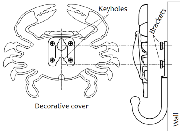
Fig. 3 Press decorative cover onto mounting bracket while pushing downward to lock in place.
