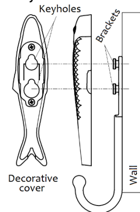
Fig. 3 Press decorative cover onto mounting bracket while pushing downward to lock in place.
