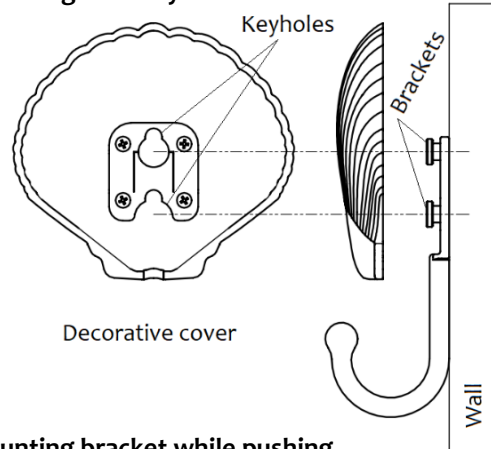
Fig. 3 Press decorative cover onto mounting bracket while pushing downward to lock in place.
